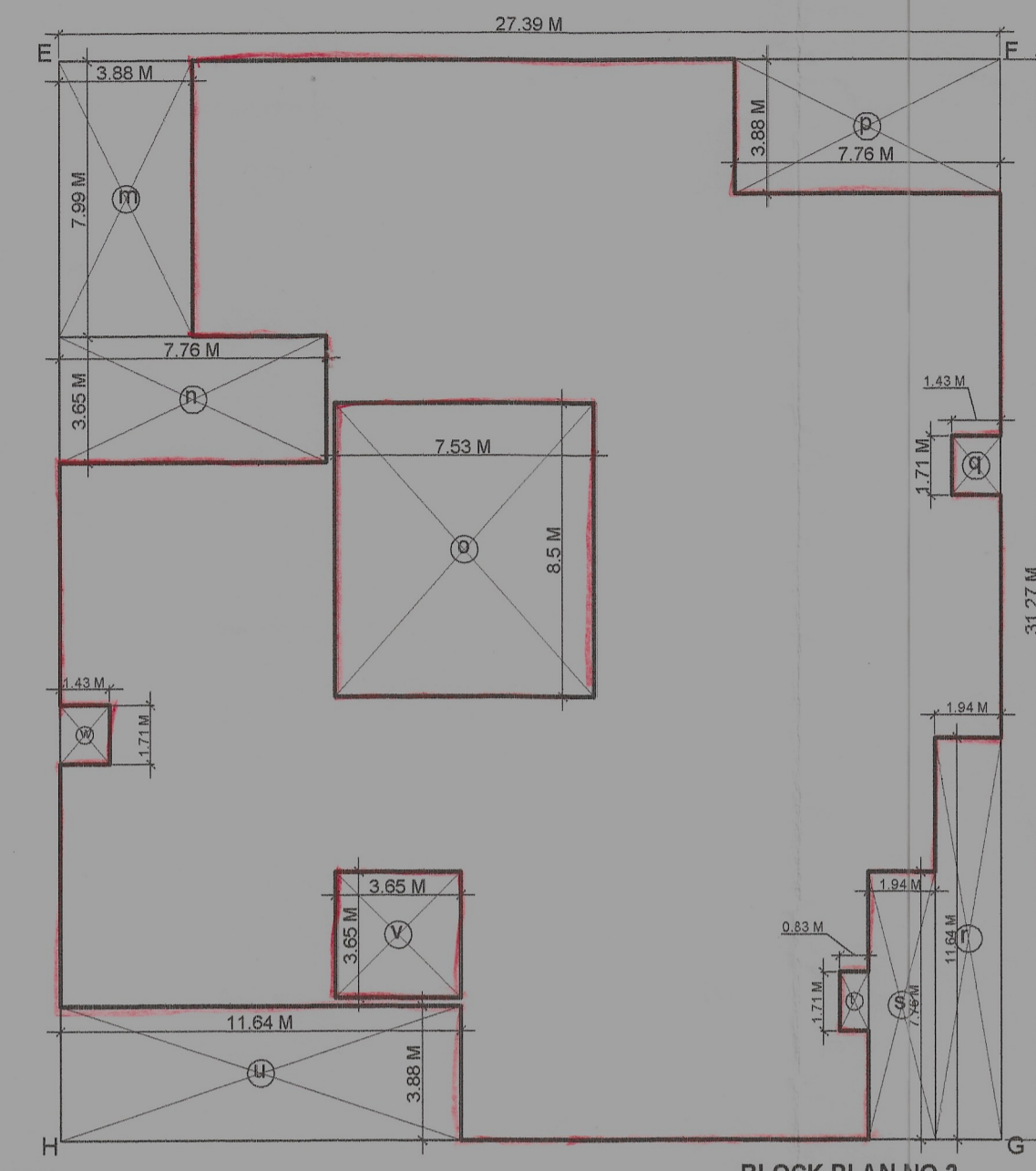
FIRST FLOOR PLAN AREA CALCULATIONS FOR FIRST FLOOR PLAN
